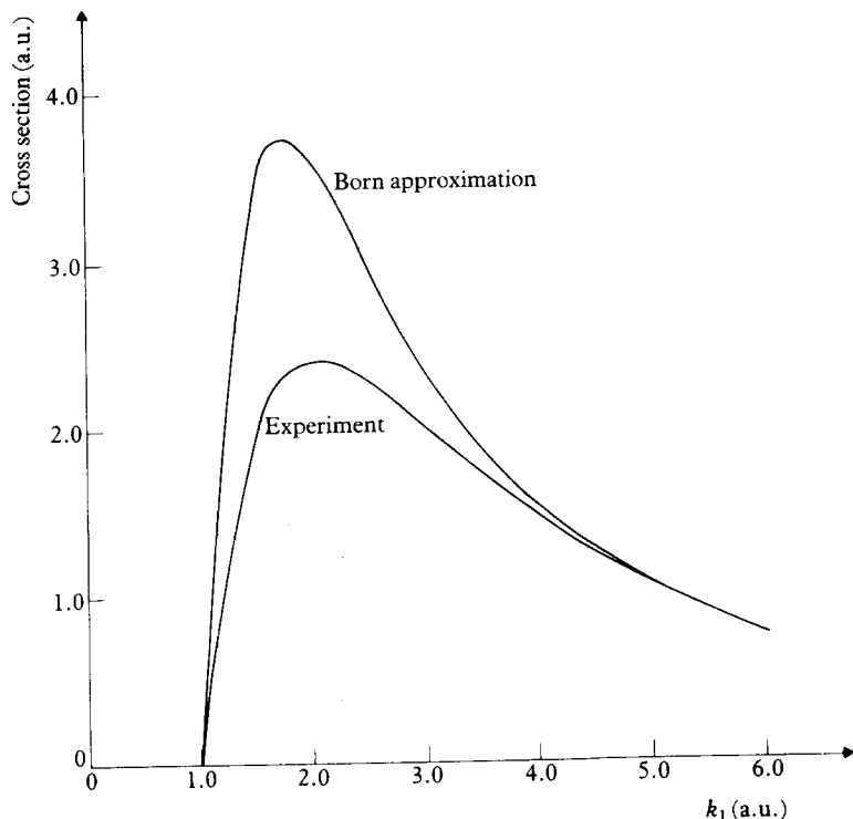
12.8 The cross-section for ionisation of atomic hydrogen by electron impact.
